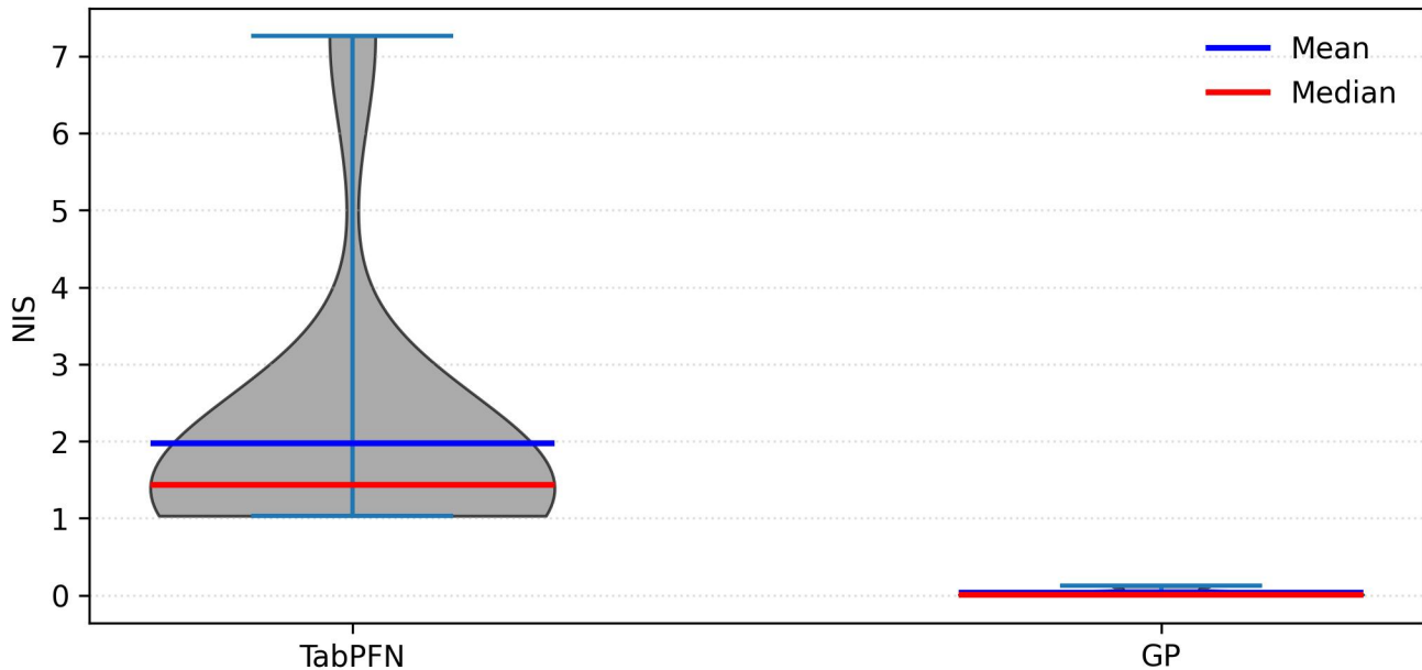
NIS distribution (n=10)
